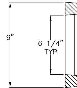
GRATE SECTION
