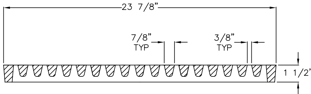
GRATE SECTION
